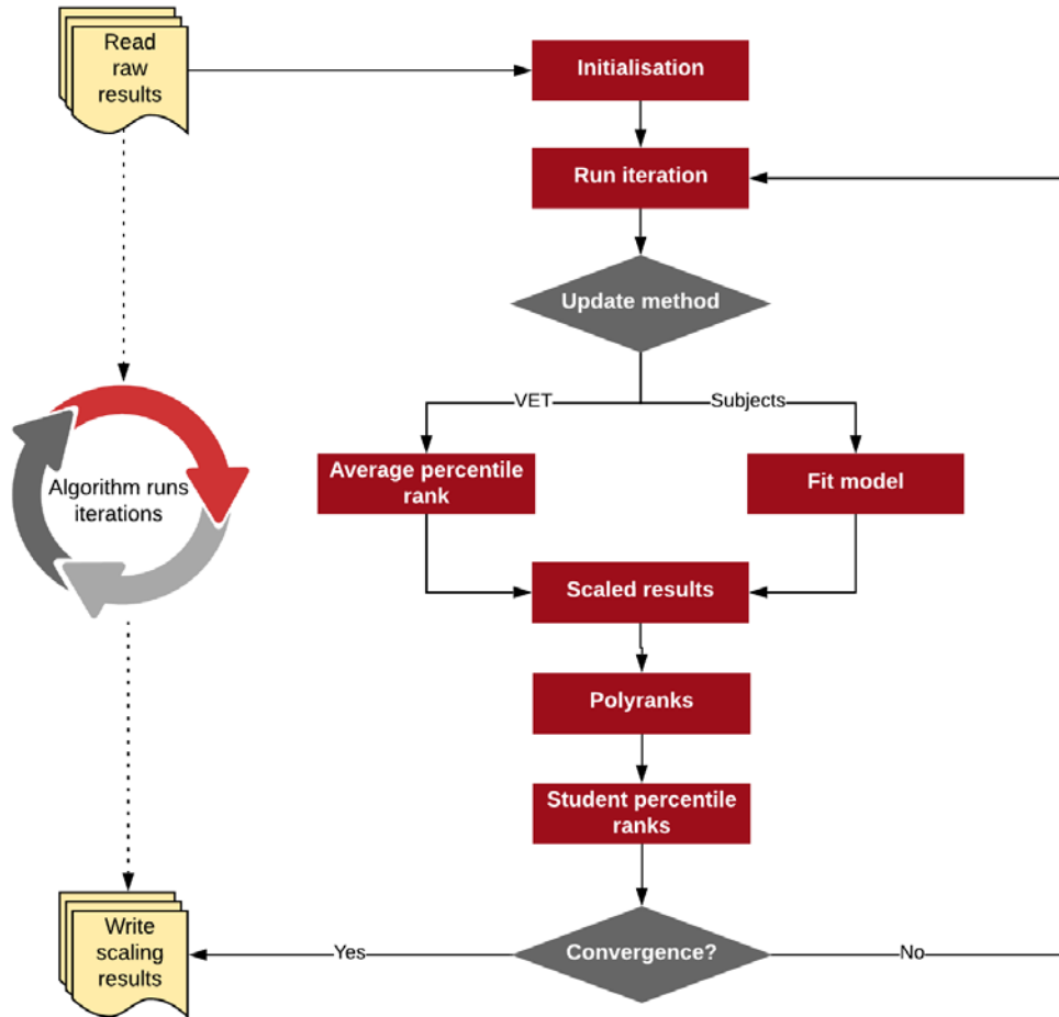
Figure 5: Algorithm Diagram
